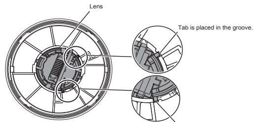
LED Unit Topside View (Attachable)
