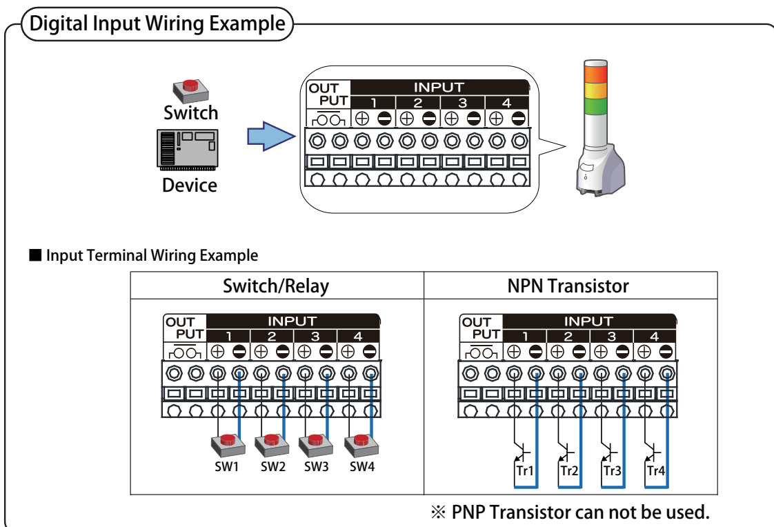
Figure 3.2.1-1 Digital Input Wiring Example
