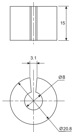
Outer Dimensions (Unit: mm)
