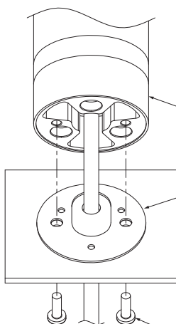
Compatible Direct Mount Bracket
